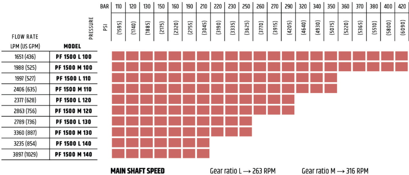
PF 1500 - 50 Hz 4 POLES ELECTRIC MOTOR (1500 RPM) - MAX ABSORBED POWER 1500 kW
