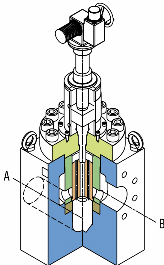
Actuated version
