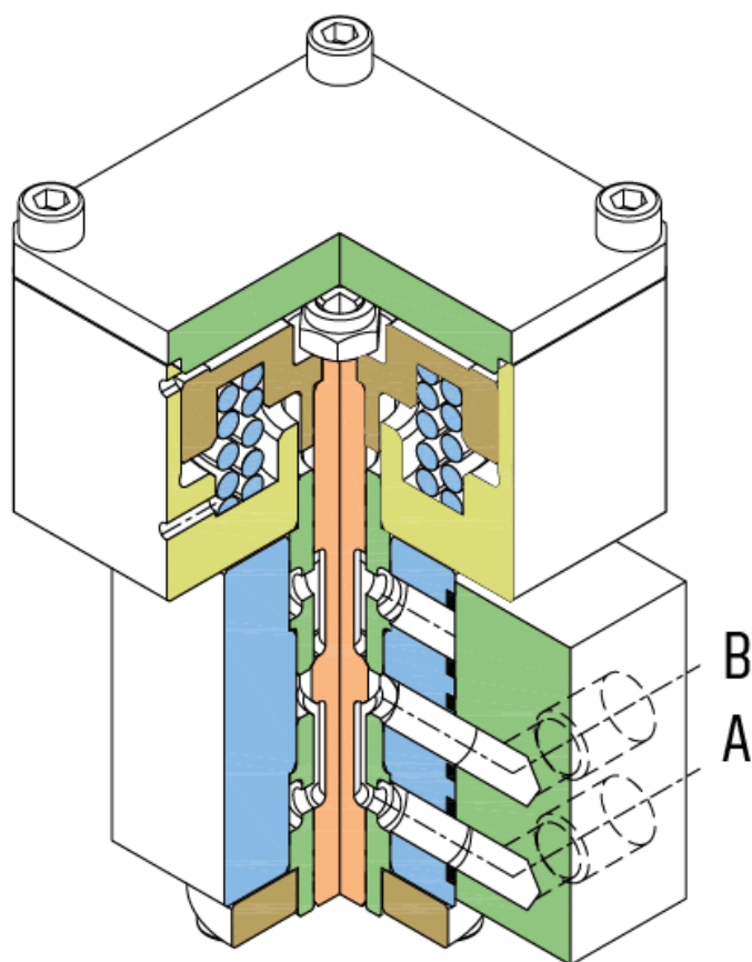
2/2-way version
